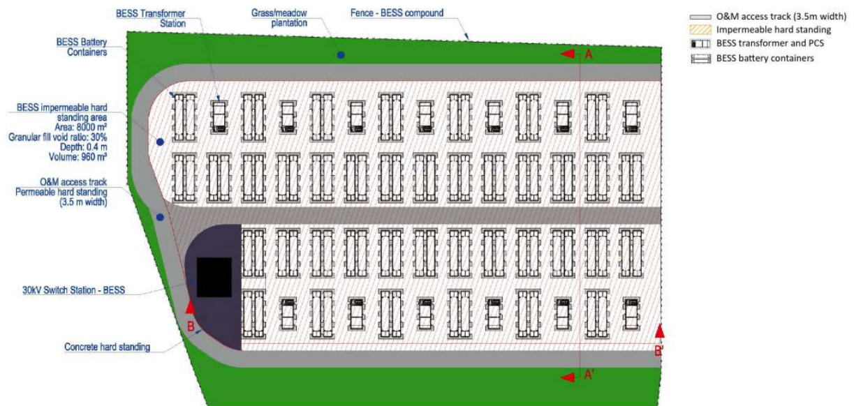
FIGURE 9.2 - INDICATIVE BESS LAYOUT
